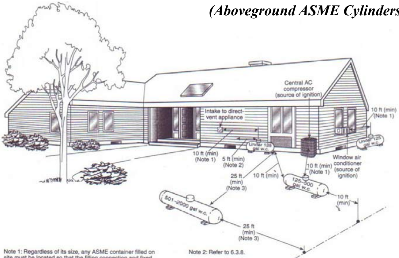
FIGURE I.1(a) Cylinders. (Figure for illustrative purposes only; code compliance required.)
